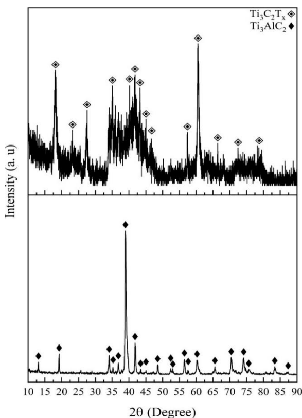
Fig. 1. X-ray diffraction patterns of \text{Ti}_3\text{AlC}_2 MAX phase a) before and b) after etching process in HF solution for 24 h
